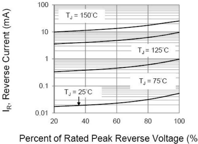
Fig.3-Typical Reverse Characteristics
